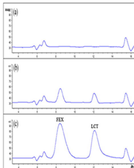
Fig. 6. HPLC chromatograms for Fexofenadine and Levocetirizine after extraction at optimum conditions (toluene as organic solvent, pH_{donor} = 2.5 , pH_{acceptor} = 12.0 , stirring rate of 1000 rpm, extraction time of 30 min, with no salt addition). (a) blank plasma sample (b) patient plasma sample and (c) 300 ng/mL spiked patient plasma sample. Mobile phase: mixture of methanol, acetonitril and 0.5% aqueous solution of triethylamine (20:30:50, v/v); flow rate: 1.0 mL/min; column: C18 (250 × 4.6 mm, 10 \mu m); \lambda = 226 nm at room temperature.
