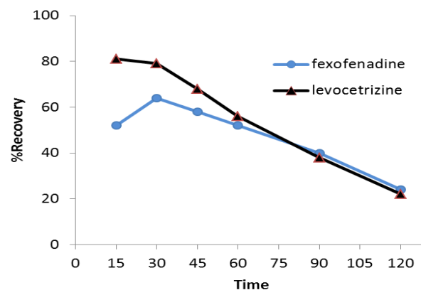
Fig. 5. Effect of extraction time on the extraction recovery of Fexofenadine and Levocetirizine. Extraction conditions: stirring rate = 1000 rpm. Other conditions as Fig. 4.
