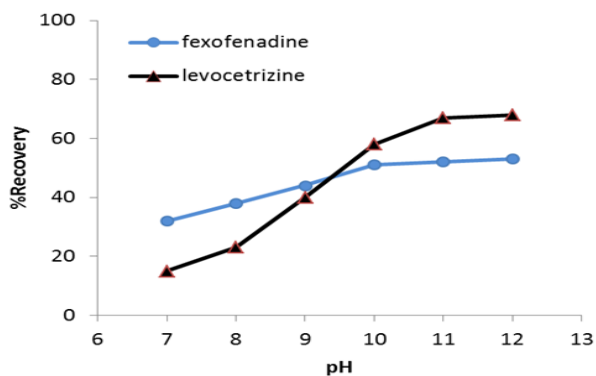
Fig. 3. Effect of the acceptor phase pH on the extraction recovery of Fexofenadine and Levocetirizine. Extraction conditions: pH donor = 2.5. Other conditions as Fig. 2.
