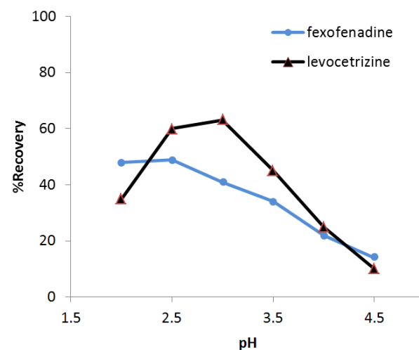
Fig. 2. Effect of donor phase pH on the extraction recovery of Fexofenadine and Levocetirizine. Extraction conditions: toluene as organic extraction solvent, donor phase, 11 mL of aqueous solution containing 0.1 µg/mL of fexofenadine and levocetirizine; extraction time = 30 min; stirring rate = 250 rpm; acceptor phase, 30 µl of 0.1 mM NaOH.
