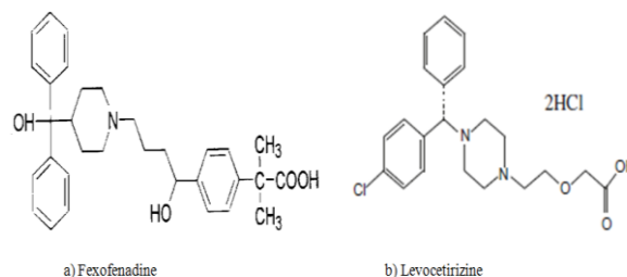
Fig. 1. Chemical structure of (a) fexofenadine and (b) levocetirizine.
