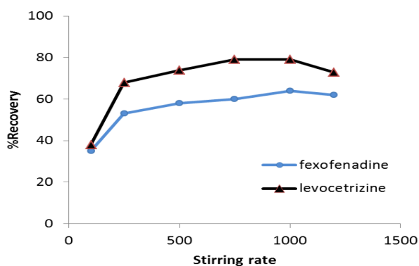
Fig. 4. Effect of stirring rate on the extraction recovery of Fexofenadine and Levocetirizine. Extraction conditions: pH acceptor = 12.0. Other conditions as Fig. 3.
