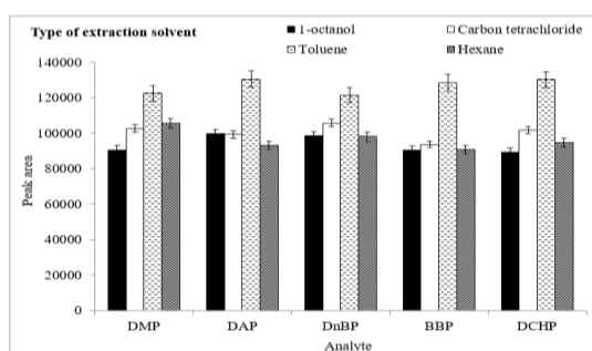
Fig. 2. The effect of extraction solvent type on MSB-LPME efficiency.
