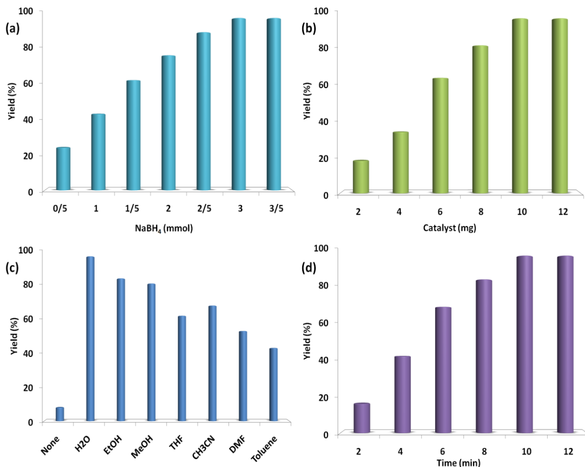
Fig. 5. Reaction the attendance of NaBH 4 amount (a), catalyst amount (b), various solvents (c), and time (d) by Nd 2 Sn 2 O 7 .
