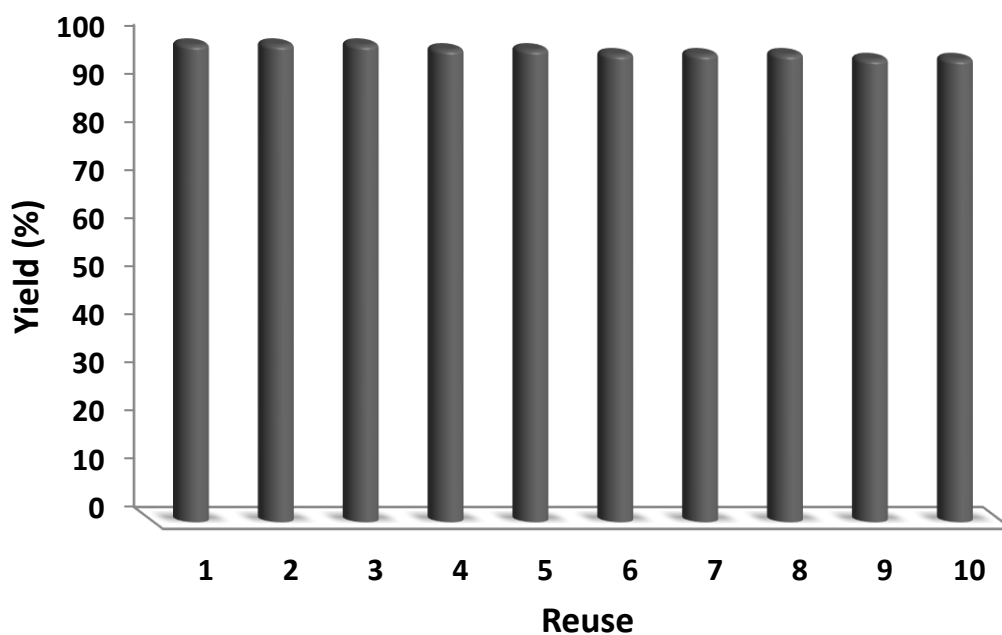
Fig.9. The reusability of \text{Nd}_2\text{Sn}_2\text{O}_7 for the reaction.
