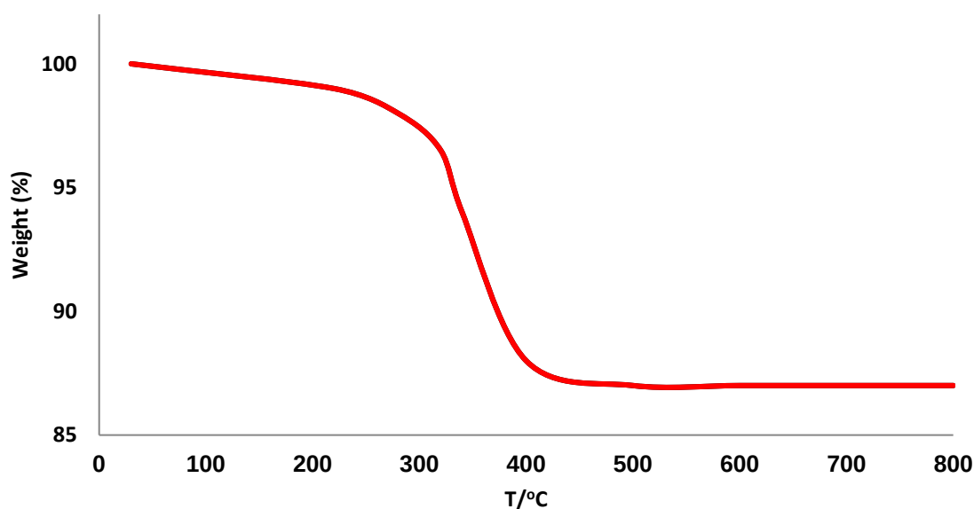
Fig. 2. TGA graph of \text{Nd}_2\text{Sn}_2\text{O}_7 .
