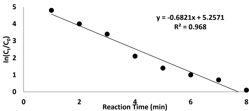
Fig. 8. The scheme of \ln(C_t/C_0) against time for the reaction over \text{Nd}_2\text{Sn}_2\text{O}_7 .
