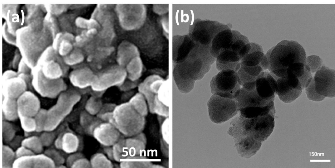
Fig. 1. FESEM (a) and TEM (b) of \text{Nd}_2\text{Sn}_2\text{O}_7 produced in the most appropriate conditions.
