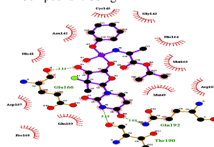
Compound f: Using MVD
