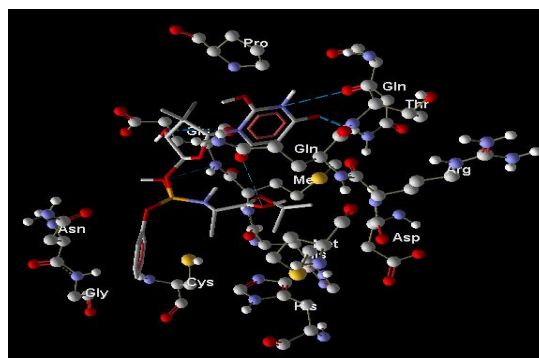
Compound f: Using MVD
