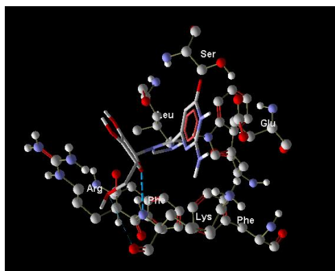
compound a: using MVD
