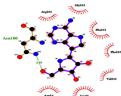
compound j: using MVD
