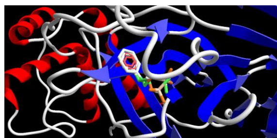
Fig. 2. Binding site refinement
