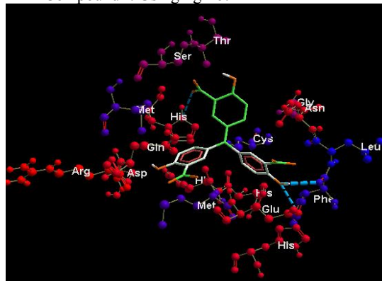
Compound k: using MVD
