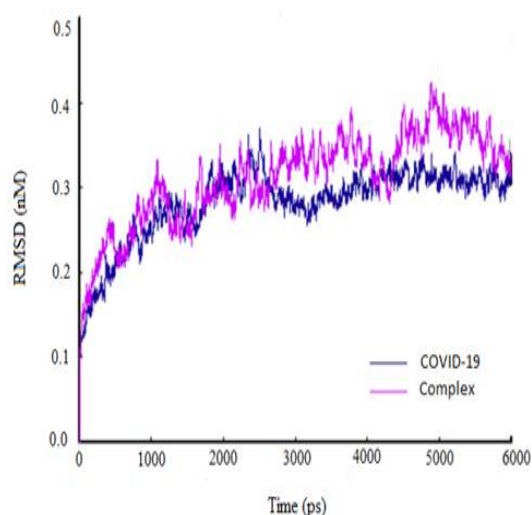
Fig. 3. RMSD values of protein backbone for COVID-19 and COVID-19 complex during 6000 ps MD simulation.
