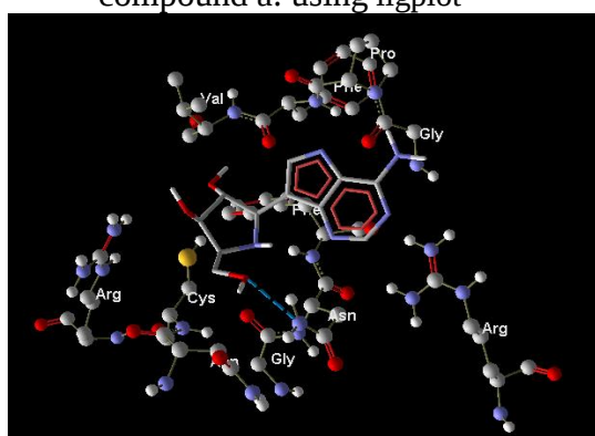
compound j: using MVD
