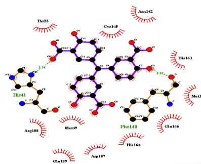
Compound k: using MVD
