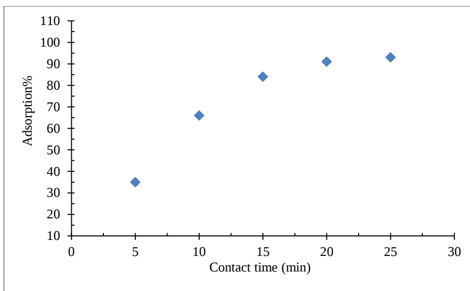
Fig. 3. Effect of contact time. Conditions: fluoride concentration (453 mg/L); \text{ZrO}_2 amount, 2.0 g; temperature, 90 °C; stirring speed, 200 rpm; pH, 6.
