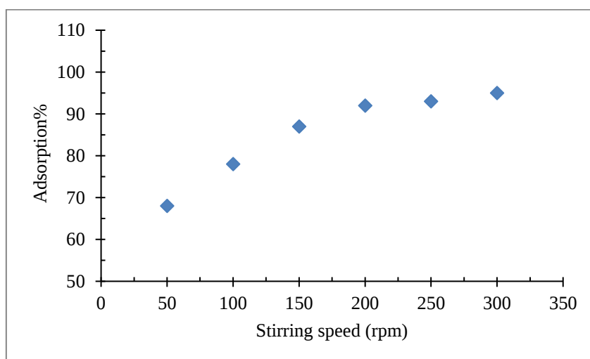
Fig. 4. Effect of stirring speed. Conditions: fluoride concentration (453 mg/L); \text{ZrO}_2 amount, 2.0 g; temperature, 90 °C; contact time, 20 min; pH, 6.
