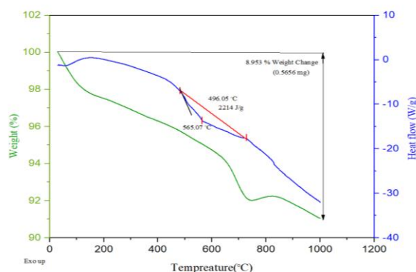
Fig. 3. TGA analysis for nanoparticles in the temperature range between 25 and 1000 °C
