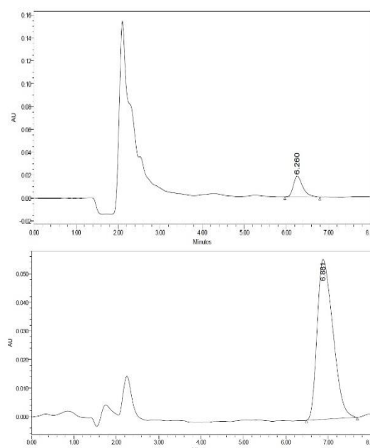
Fig. 10. HPLC chromatograms obtained for (a) non-spiked real sample of bisphenol A and (b) real sample spiked with 1 \text{ ng mL}^{-1} of bisphenol A.
